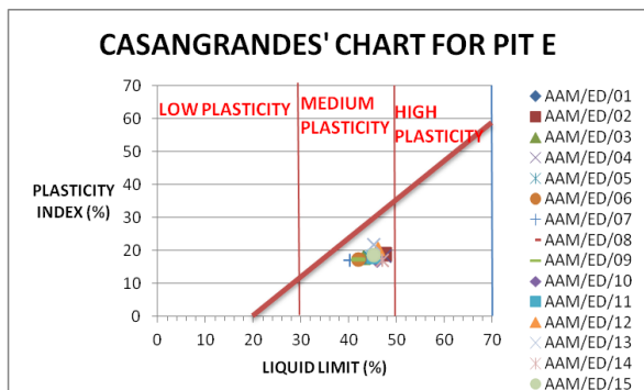
Figure 4E: Casagrande chart for pit E
