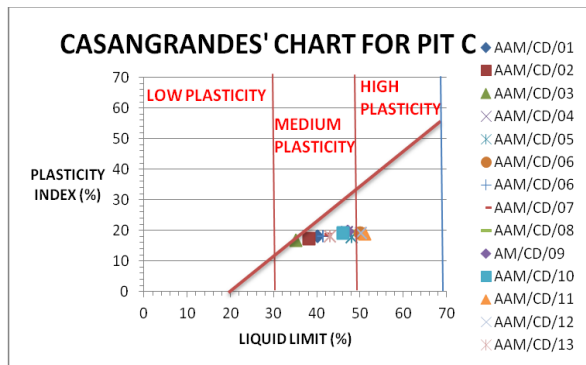
Figure 4C: Casagrande chart for pit C
