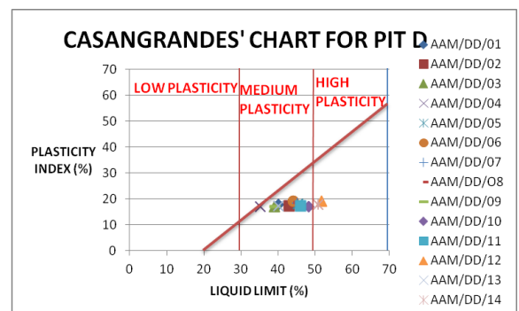
Figure 4D: Casagrande chart for pit D
