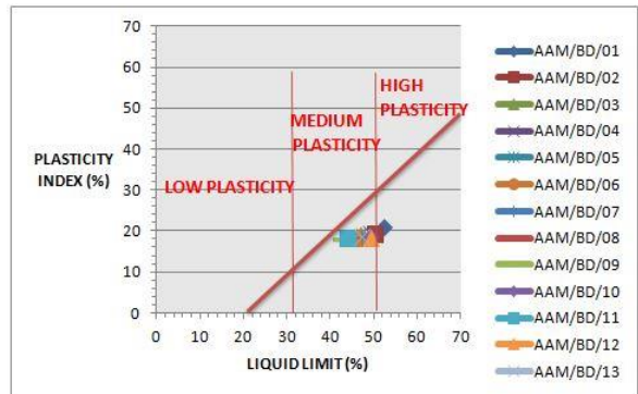
Figure 4B: Casagrande chart for pit B
