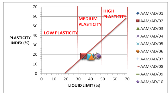
Figure 4A: Casagrande chart for pit A
