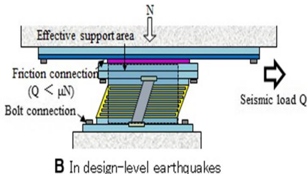
Figure 8: LRB horizontal deformation at design seismic loads
