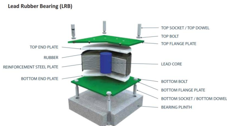
Figure 10: 3D view of LRB
